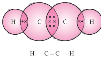
Ethyne \text{C}_2\text{H}_2
